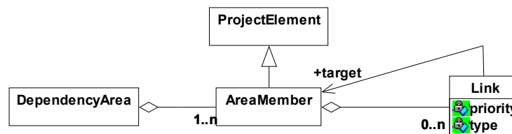
Fig. 5. The core of the Dependency Area metamodel
