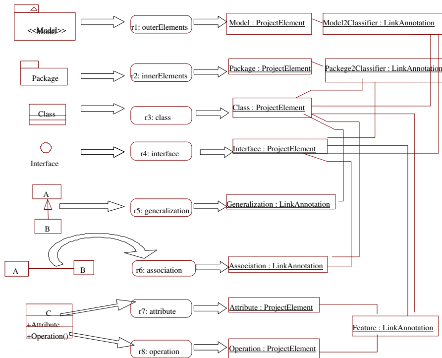
Fig. 6. Examples of transformation rules from a UML model to Project elements
