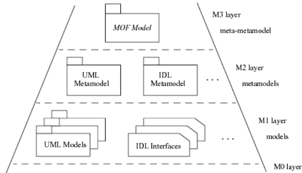
Fig. 1. The role of the MOF in the metamodel hierarchy
