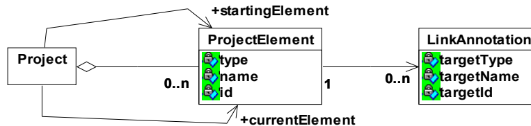
Fig. 4. The core of the Project metamodel
