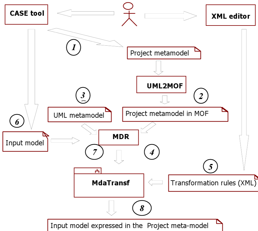
Fig. 7. Realization of the input transformation process
