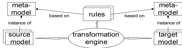
Fig. 2. Idea of model transformation in QVT
