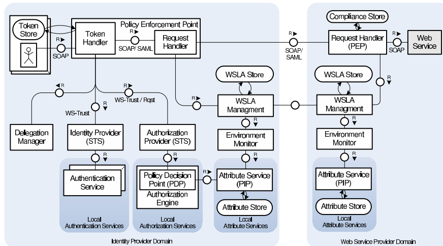
Fig. 5. The 2LAC Security Architecture
