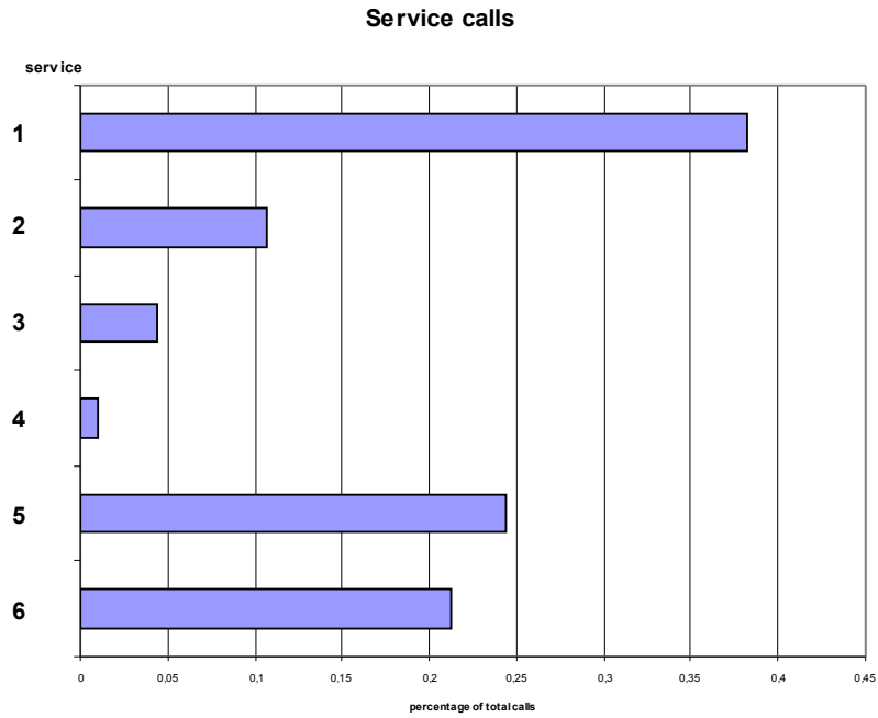
Fig. 4. The percentage of six flows in total traffic
