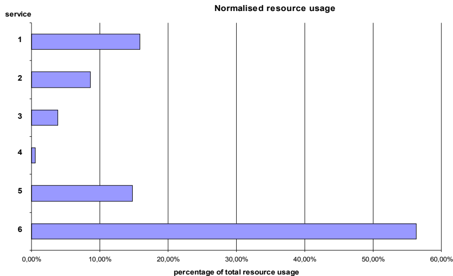
Fig. 6. The usage of server resources by selected services
