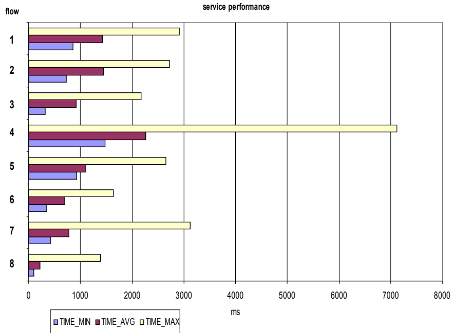
Fig. 3. Comparison of effectiveness of flows
