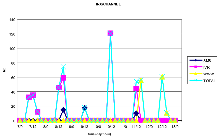
Fig. 5 Traffic in the integrated system in some time period
