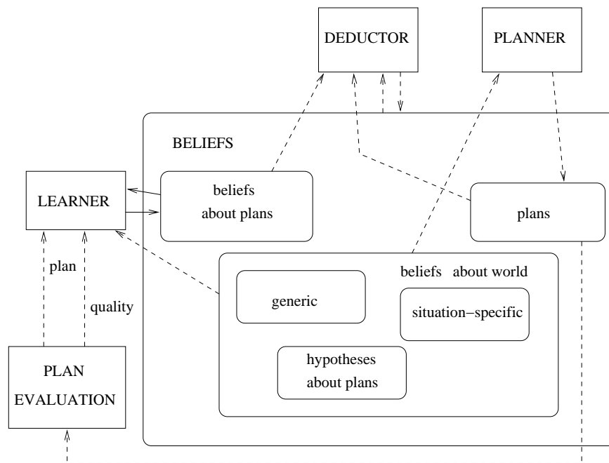
Fig. 2. Some details of the architecture of the agent.
