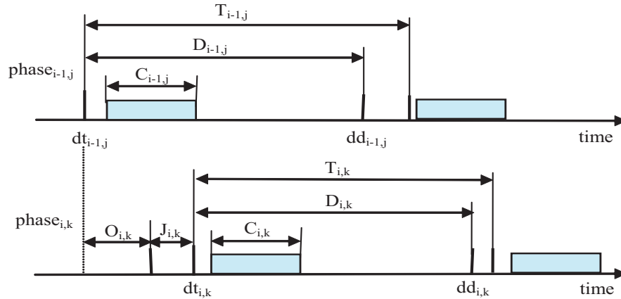
Fig. 2. Temporal relations between phases of two consecutive intersections.
