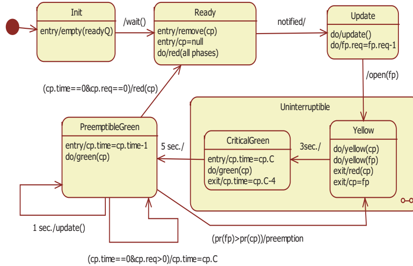
Fig. 5. Time driven dispatcher UML state machine.
