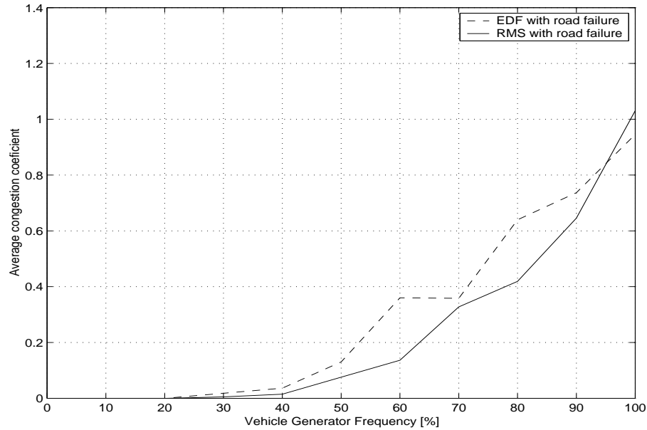
Fig. 7. System congestion degree with a traffic incident.
